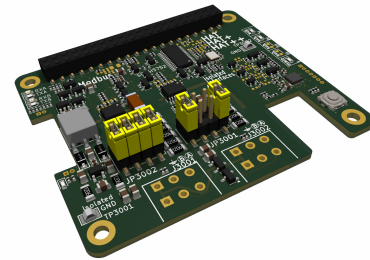
Figure 6: JP3001 / JP3002 intermediate-node configuration. LEFT: 120 \Omega termination and 5 k \Omega bias enabled. Right: Bias enabled only (termination disabled) – uncommon but valid.
